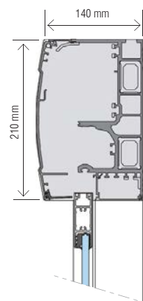
Reinforced Casing
